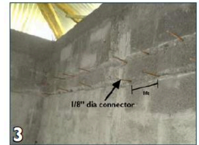
3 Insert connectors at every 1 ft.
