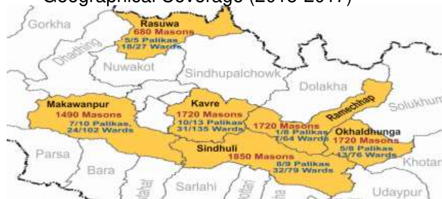
Geographical Coverage (2015-2017)
