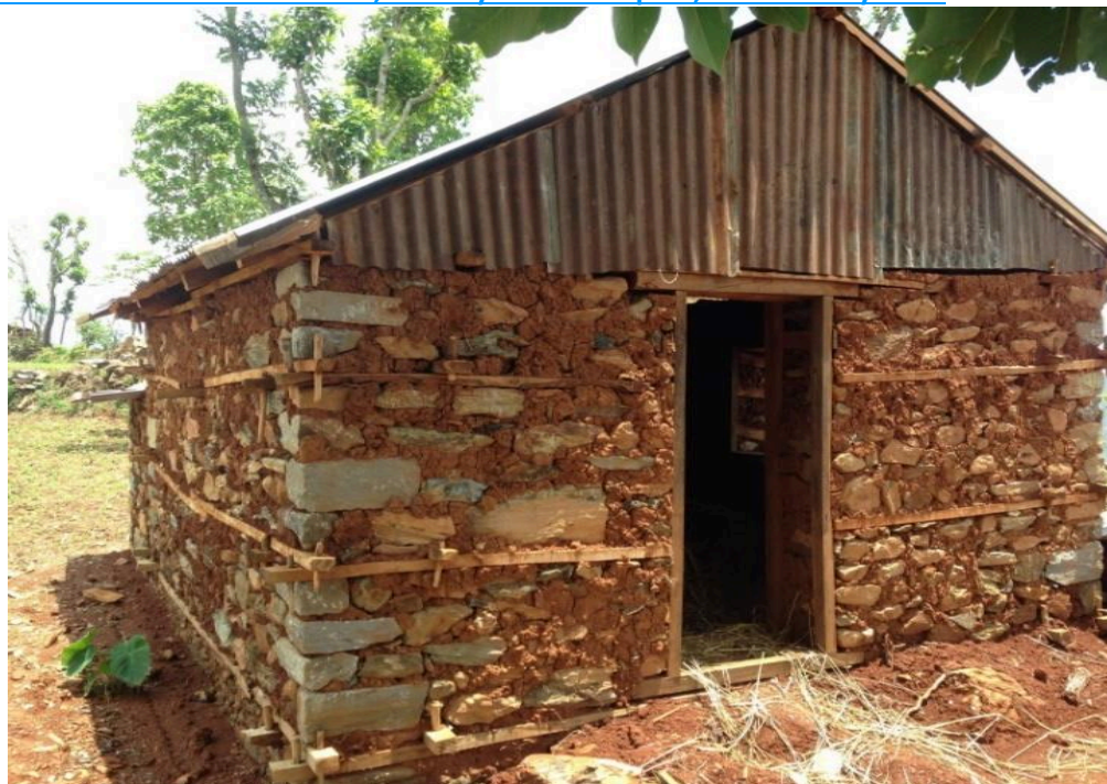
Ward No. 8, Bidur Municipality, Nuwakot: a stone and mud mortar house with timber bands. The house belongs to a vulnerable family. The home owner has received the second tranche of the GoN housing reconstruction grant and will be recommended for third tranche after shuttering.
