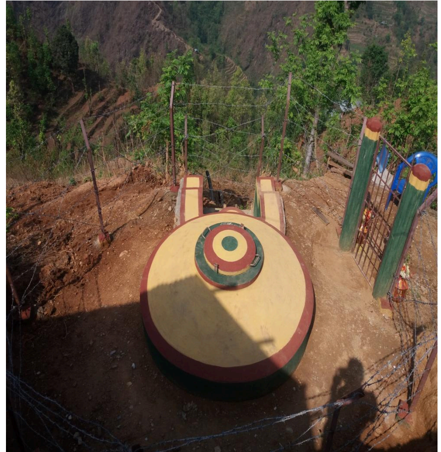
RVT Construction at Adamara WSS
