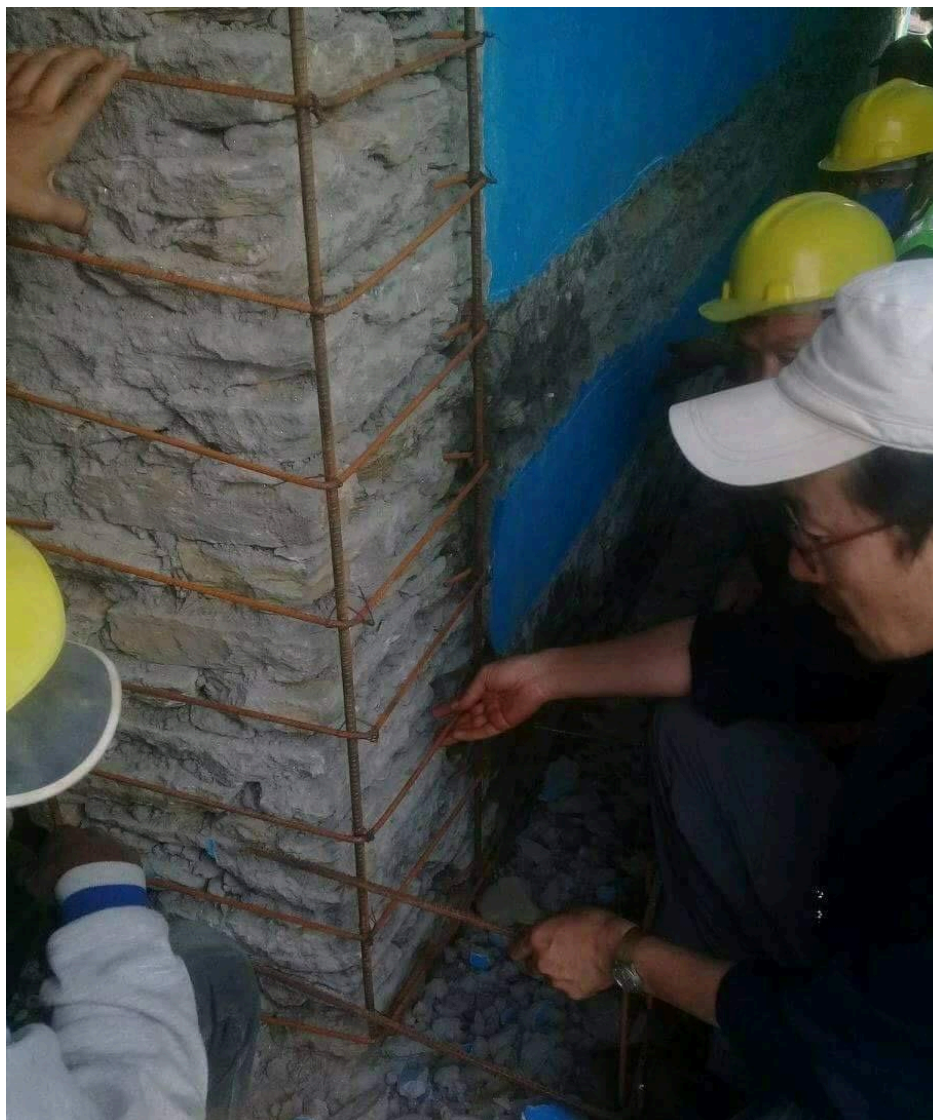
Correction and retrofitting in Barpak, Gorkha. Photo Credit: Er. Mahendra Sahi Thakuri.
