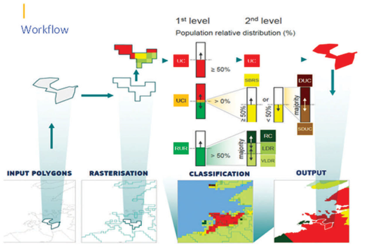
Figure 5: Workflow of DEGURBA Tool
