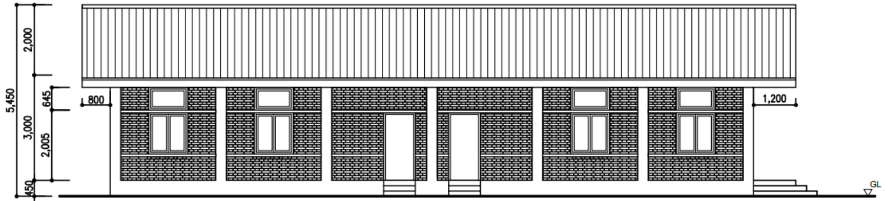
Side Elevation
