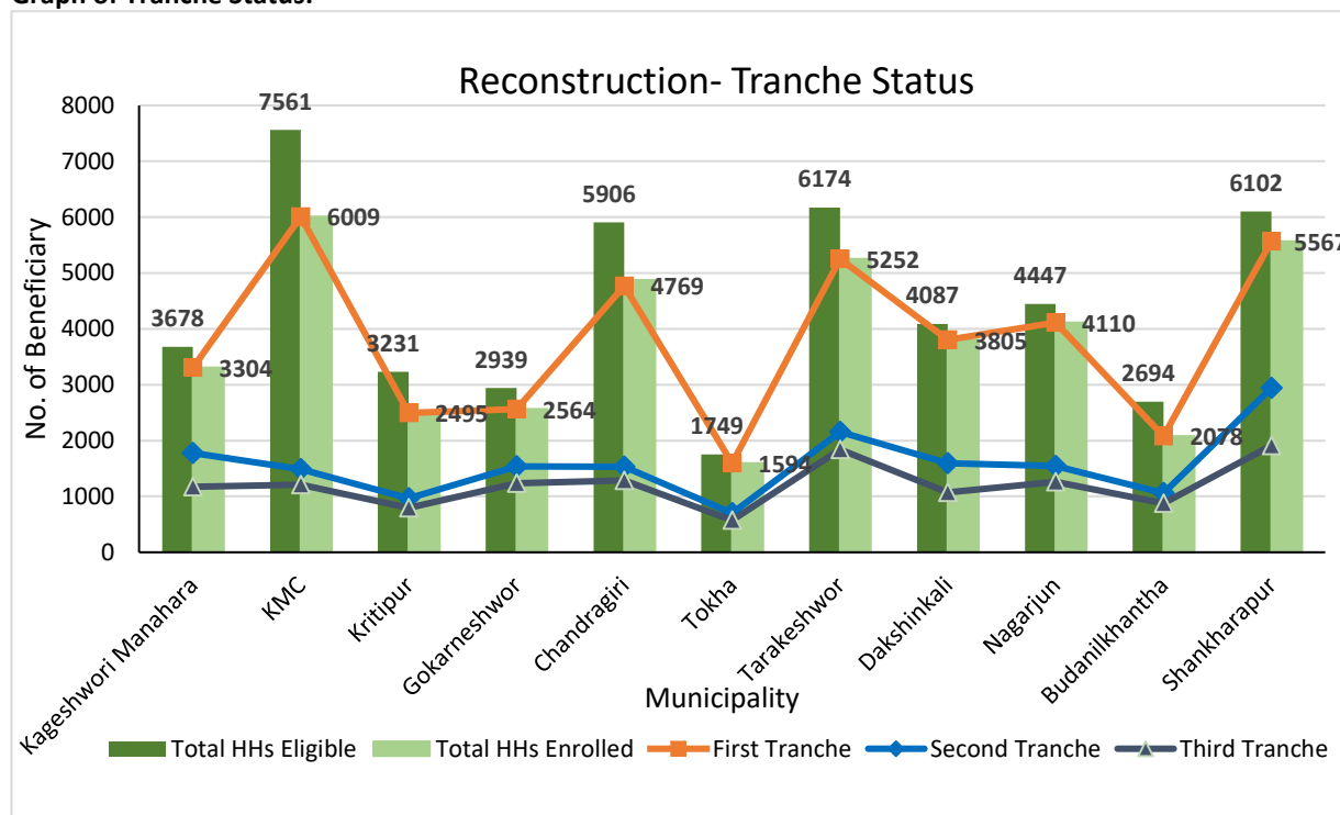
Graph of Tranche Status:
