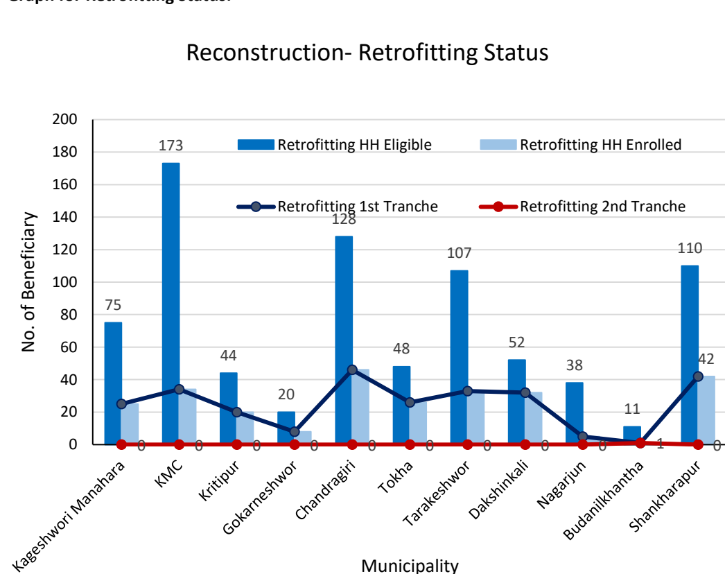
Graph for Retrofitting Status:
