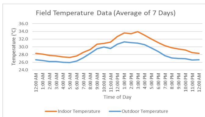
Figure 17 Temperature Variation ( Field Measurements)
