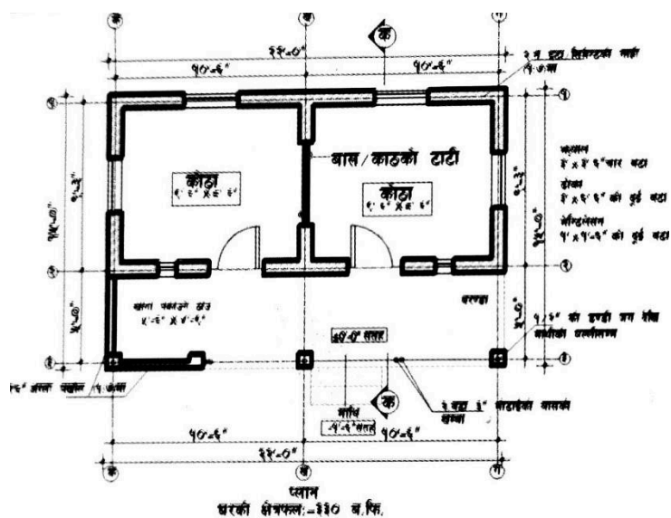
Figure 13 House Plan for Terai Region
