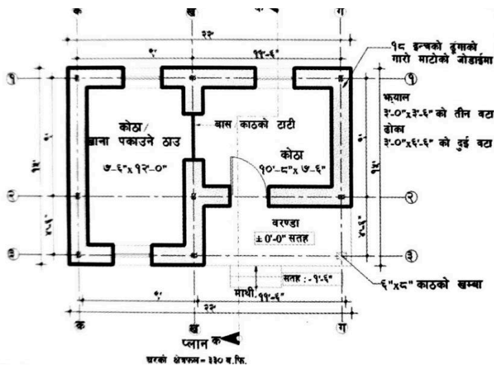
Figure 12 House Plan for Inner Madhesh, Hills and Mountain Region
