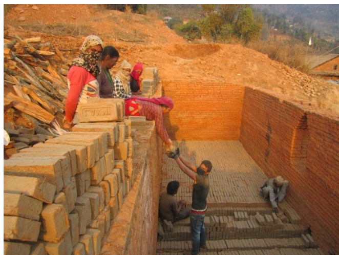
Preparations to burn bricks at temporary brick kiln, Bhumlutar
