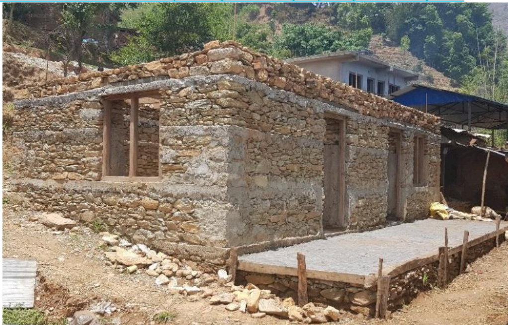
Ward No. 3, Suryagadhi Rural Municipality, Nuwakot: a two room, stone and mud mortar masonry house. The home owner has received the second tranche of the GoN housing reconstruction grant.
