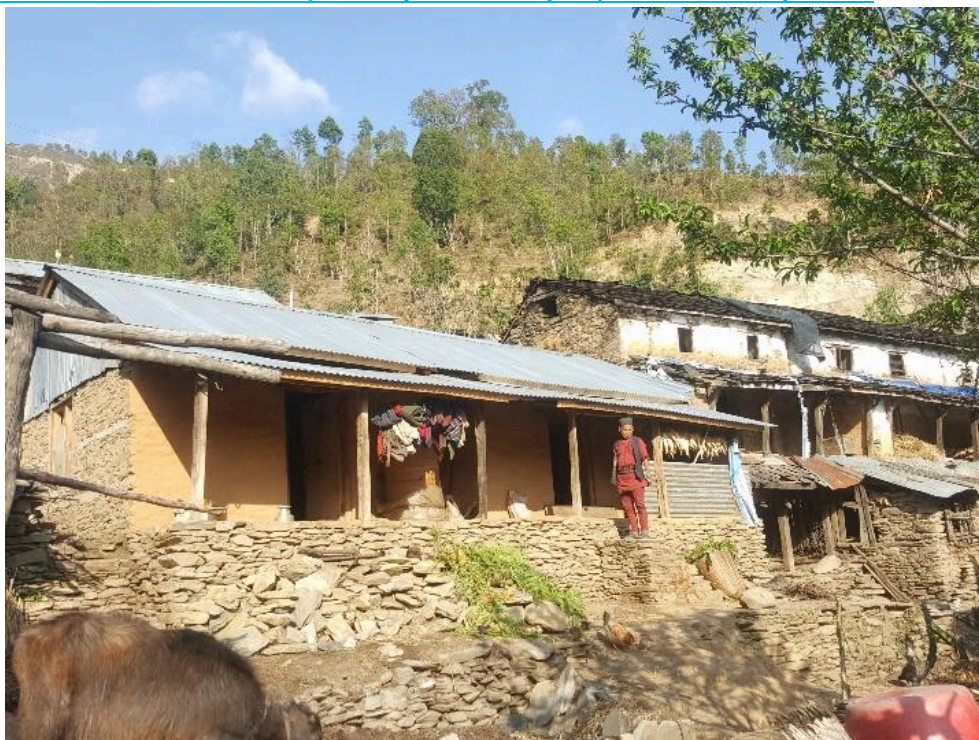
Ward No. 3, Naukunda Rural Municipality, Rasuwa: load bearing, stone and mud mortar masonry with RCC bands. Two single room houses, belonging to father and son. There is a gap in between the houses but they have a common roofing. Both the home owners have received all three tranches of the GoN housing reconstruction grant.
