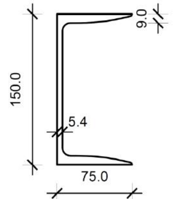
ISMC150 (SECONDARY BEAM)
