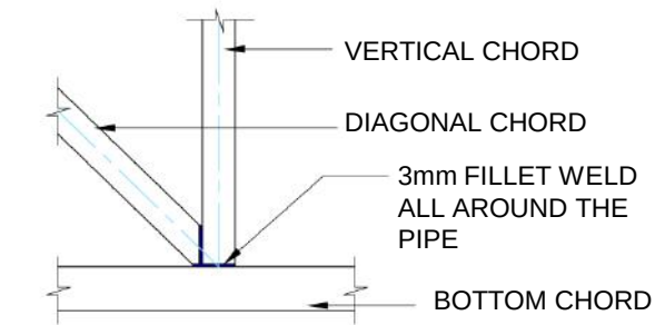
DETAIL AT A
