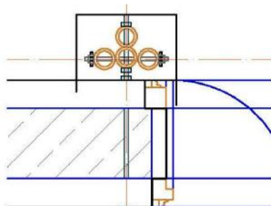
DETAIL B (PLAN): BASE PAD FOR BAMBOO CLUSTER POSTS 'TYPE 1' AND TYPE 2'
