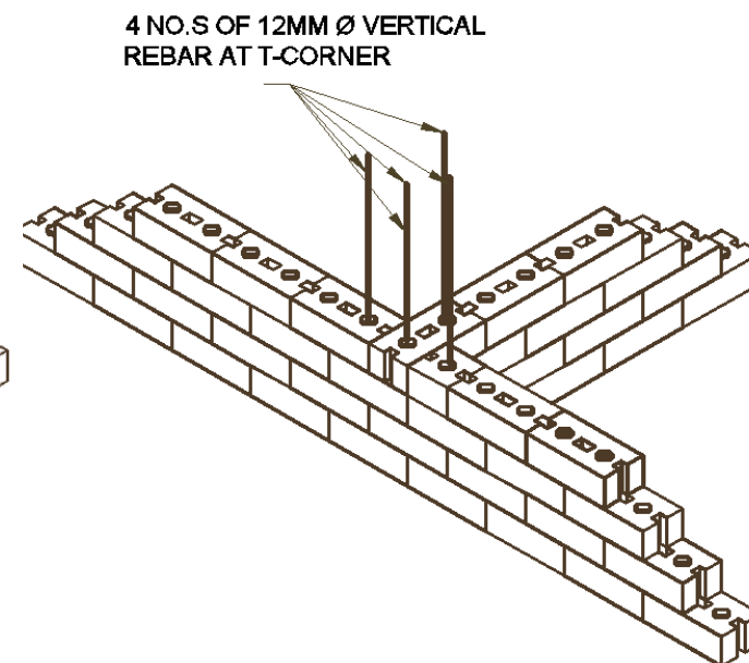
DETAIL B (TYPICAL DETAIL OF T-CORNER)
