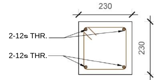
TIE BEAM
