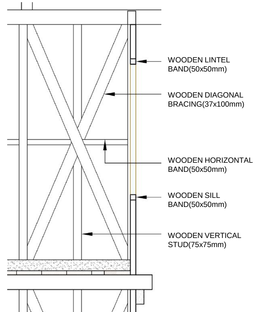
BRACING DETAIL AT A
