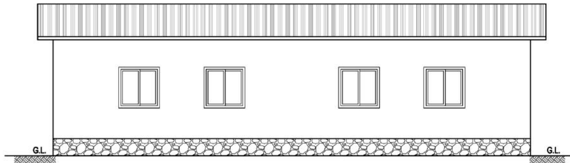
BACK ELEVATION
