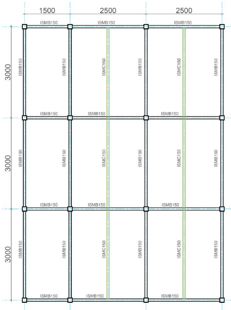
BEAM-COLUMN PLAN
