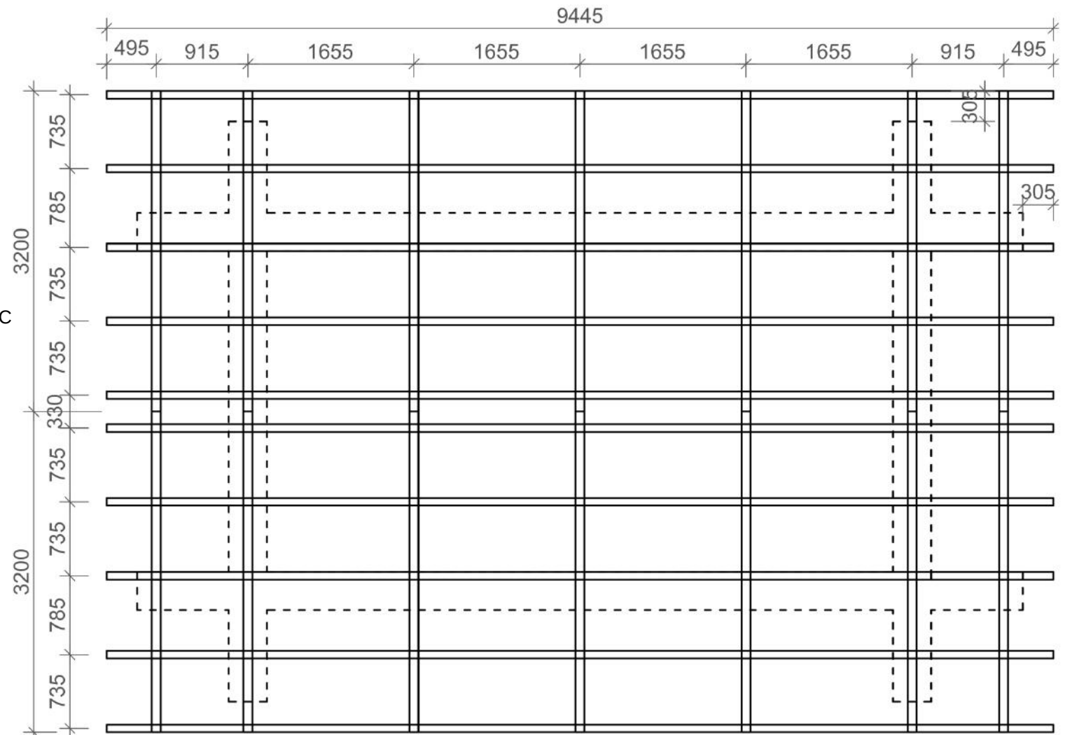
ROOF PLAN
