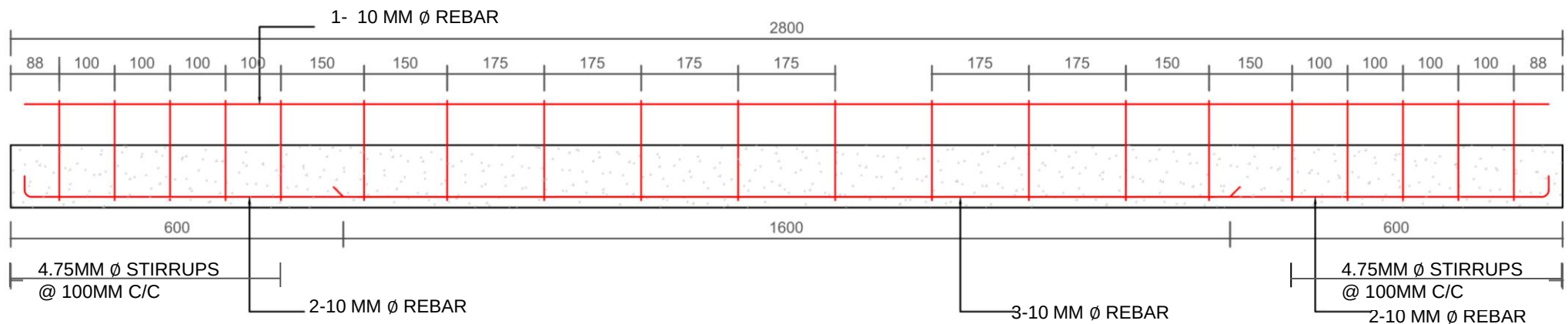
LONGITUDINAL SECTION OF PRECAST BEAM
