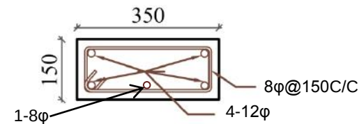
PLINTH BAND
