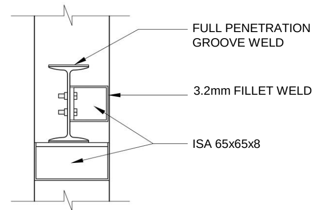
BEAM AND COLUMN CONNECTION
