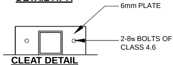
DETAIL AT A
