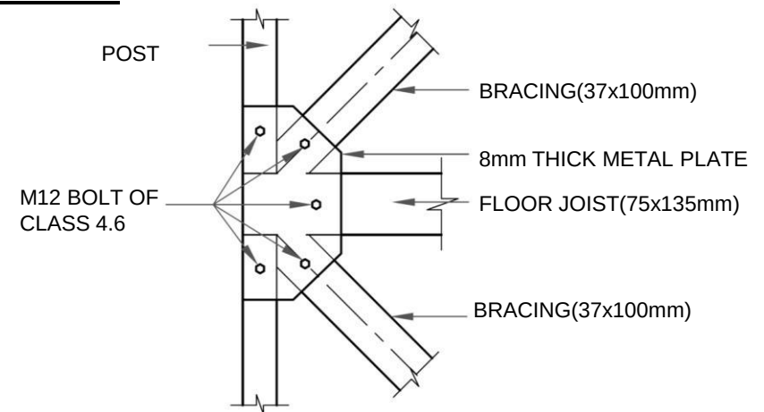
BRACING CONNECTION
