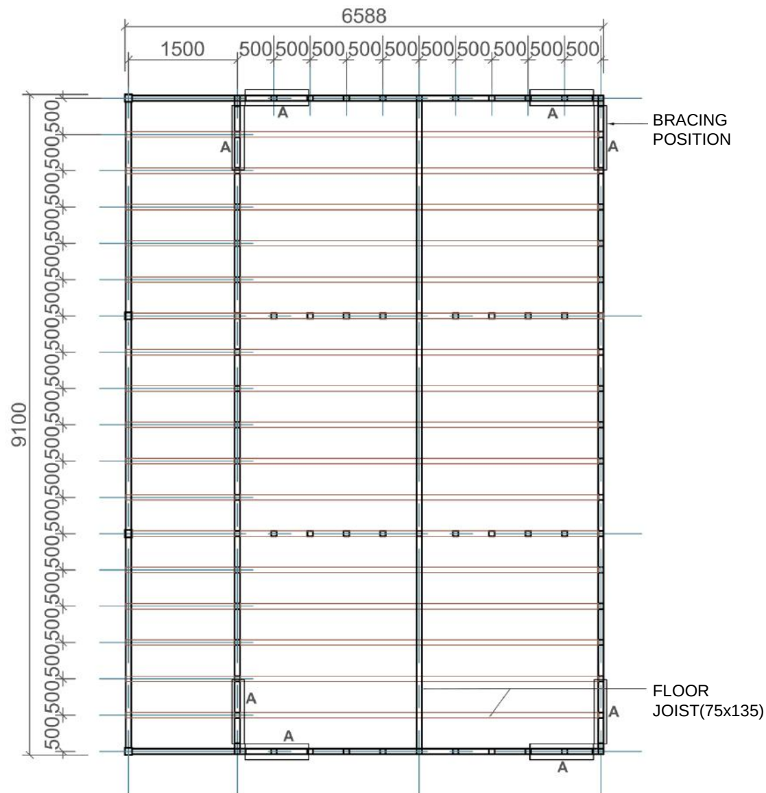
FLOOR JOIST PLAN
