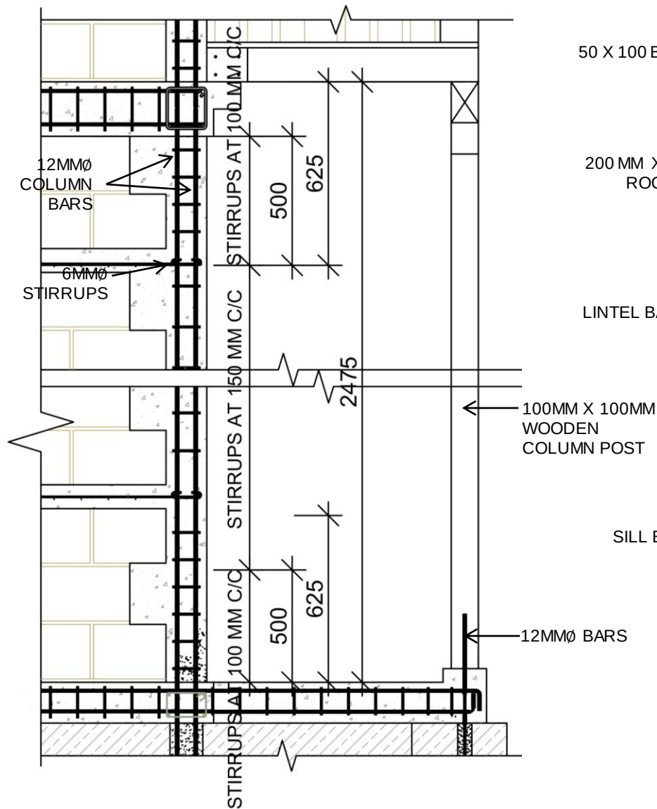
TYPICAL COLUMN SECTION: FROM GL TO FIRST FLOOR
