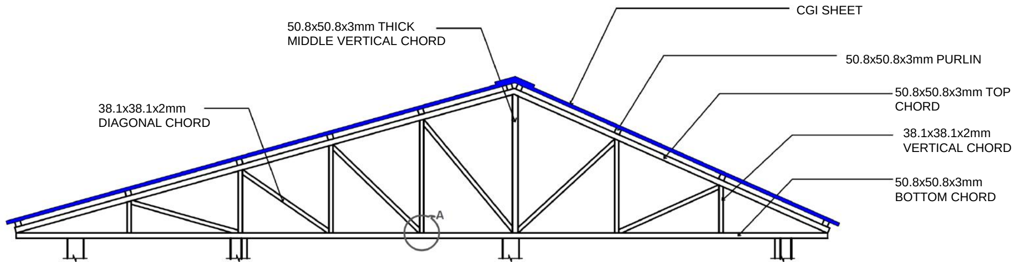
TRUSS DETAIL
