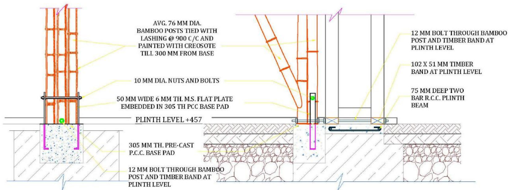
DETAIL B (SIDE ELEVATION): BASE PAD FOR BAMBOO CLUSTER POSTS 'TYPE 1' AND TYPE 2' ADAPTED FROM: RE-CONSTRUCTION OF MULTI-HAZARD RSISTANT HOUSES FOR THE 2008 KOSI AFFECTED DISTRICTS IN WEST BIHAR. PART - II: TECHNICAL GUIDELINES FOR BAMBOO BASED CONSTRUCTION
