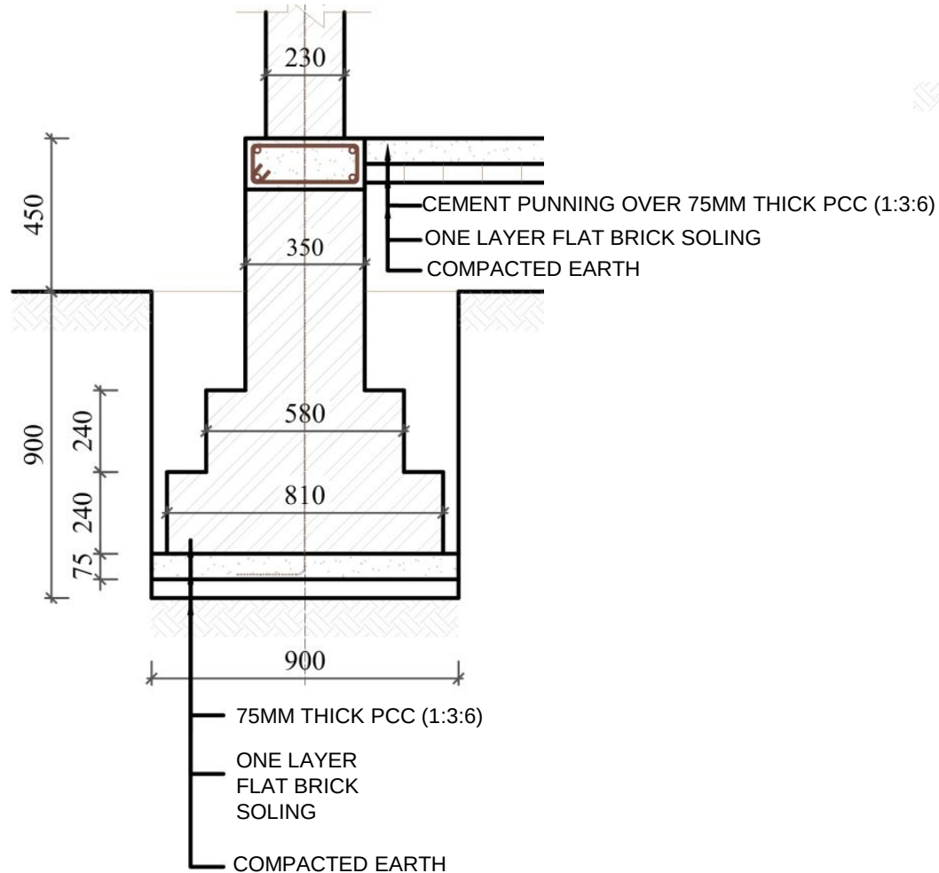
FOUNDATION SECTION
