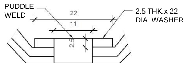
LAP DETAIL
