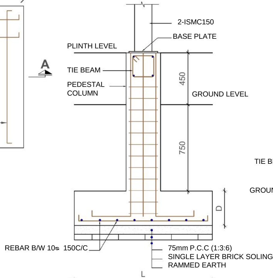
FOUNDATION SECTION AT A-A
