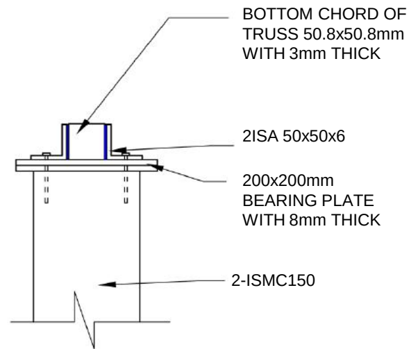
SECTION AT 1-1
