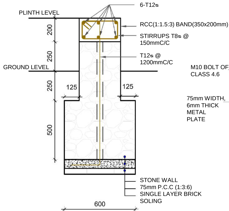
FOUNDATION
