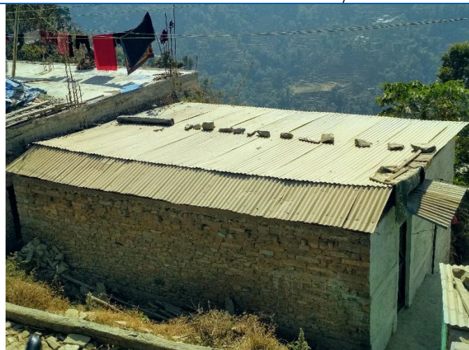
Caption: Yogendra Bhatta's stone masonry mud mortar house in Bhimsen Thapa rural municipality ward no. 1, Masel. The house is constructed without any bands and vertical reinforcement. This house has been forwarded for structural analysis and the house owner has not received second and third tranche.
