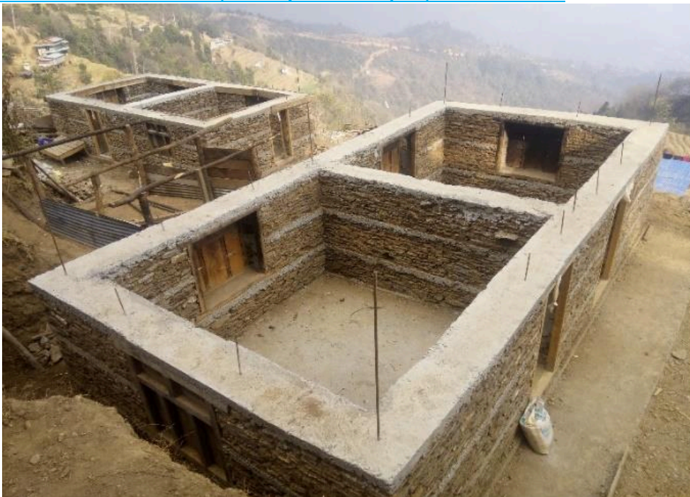
Jiri Municipality, Ward No. 4, Dolakha: a two room, one-storey, stone and mud mortar masonry home under construction. The home owner has received the first and second tranches of the GoN housing reconstruction grant.
