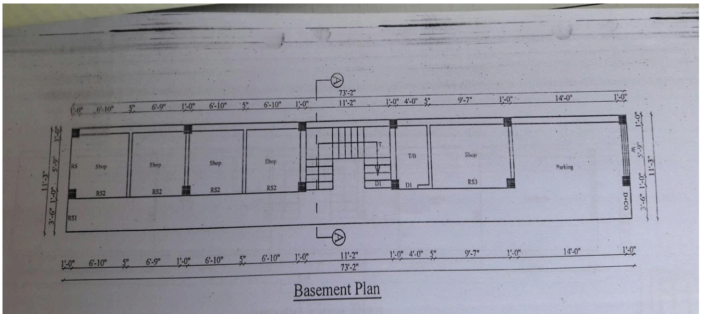
1 Bay Building (11'3"x73') Four Storey building
