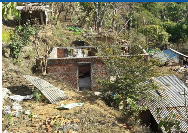
Caption: Nirmala Kattel's brick masonry cement mortar house in Gorkha urban municipality ward no. 8, Katteldanda. The house owner has received second tranche.
