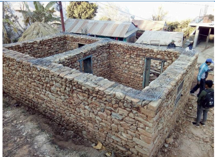
Caption: Dil kumari Gurung's stone masonry mud mortar house with guided wire mesh band in Gandaki rural municipality ward no. 2, Tanglichowk. The house is constructed with guided wire mesh in bands. This house has been constructed with the technical support of ODRC/UNDP
