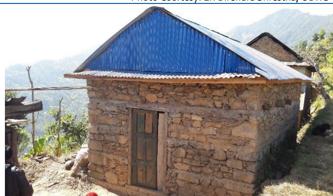
Caption: Mr. Kalu Pariyar's stone masonry mud mortar with RCC band house in Siranchowk rural municipality ward no 7, Shreenathkot. The house owner has received third tranche. The house owner received construction material support from Asal Chhimeki Nepal (ACN)
