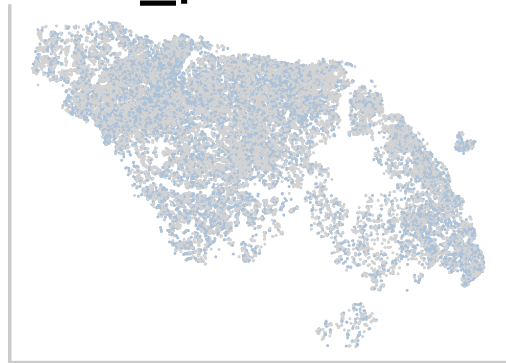
B_plasma
