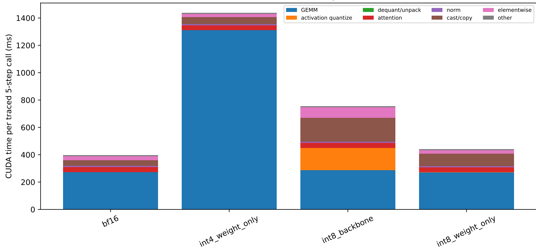
torchao kernel time decomposition
