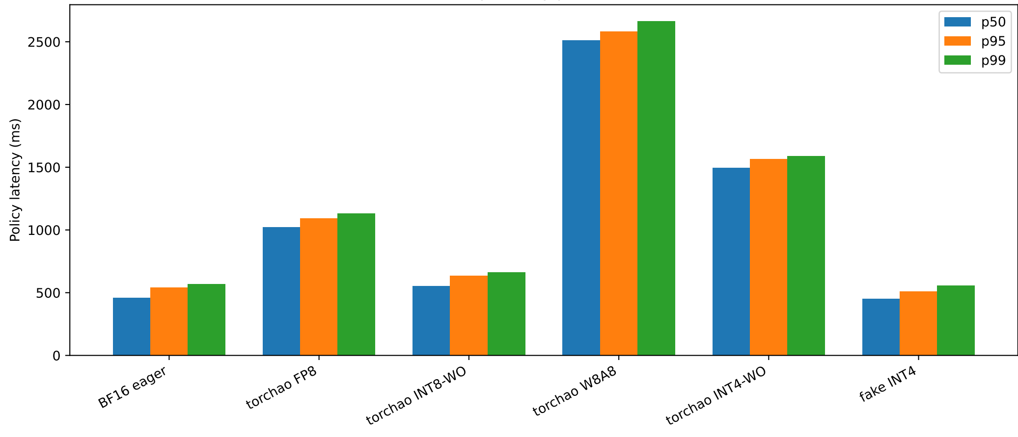
Policy latency percentiles
