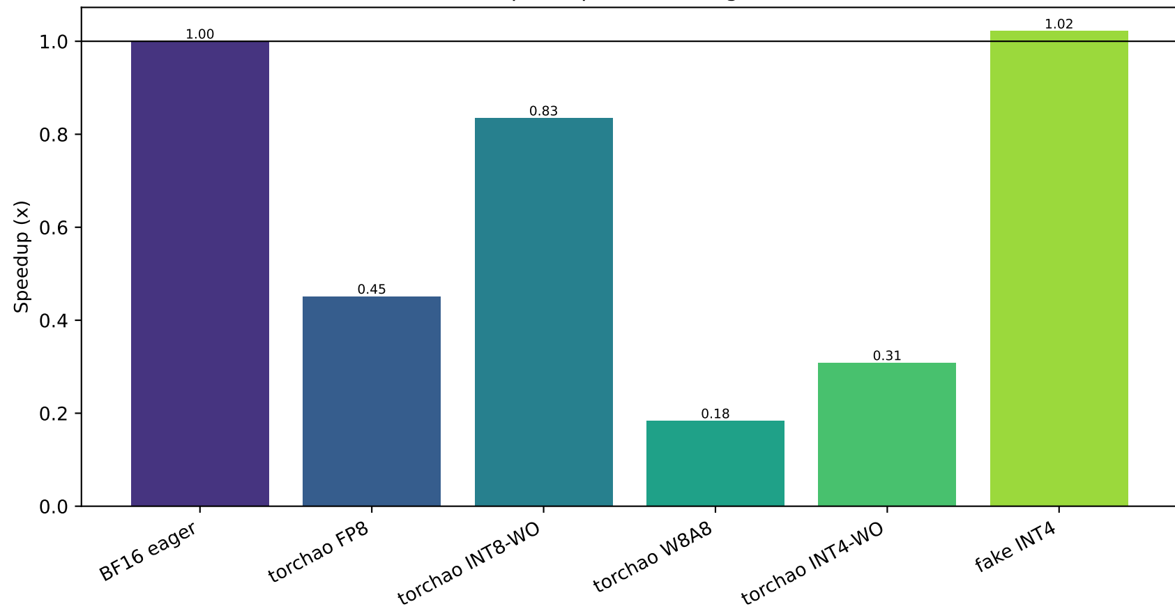
Speedup vs BF16 eager
