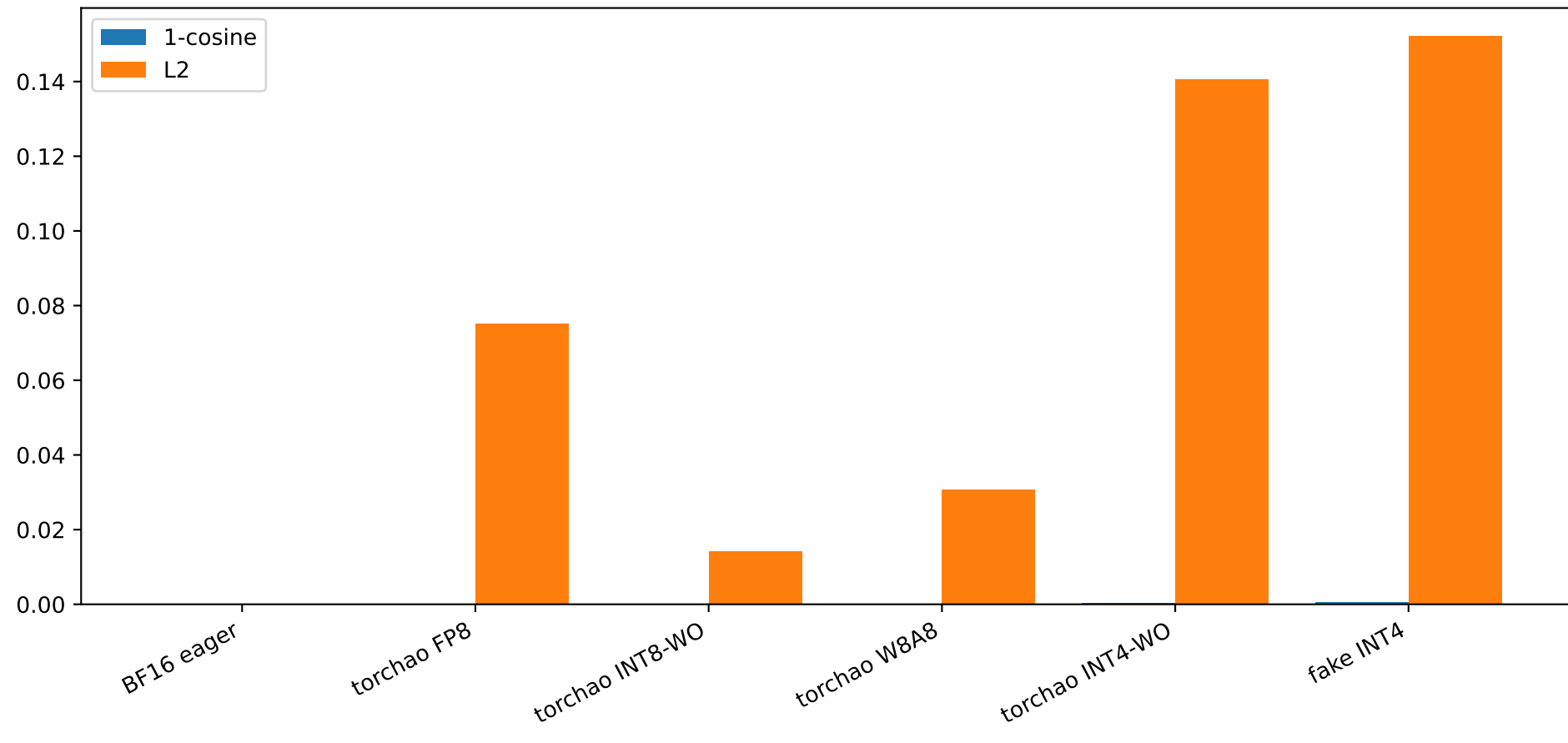
Action cosine/L2 error vs BF16
