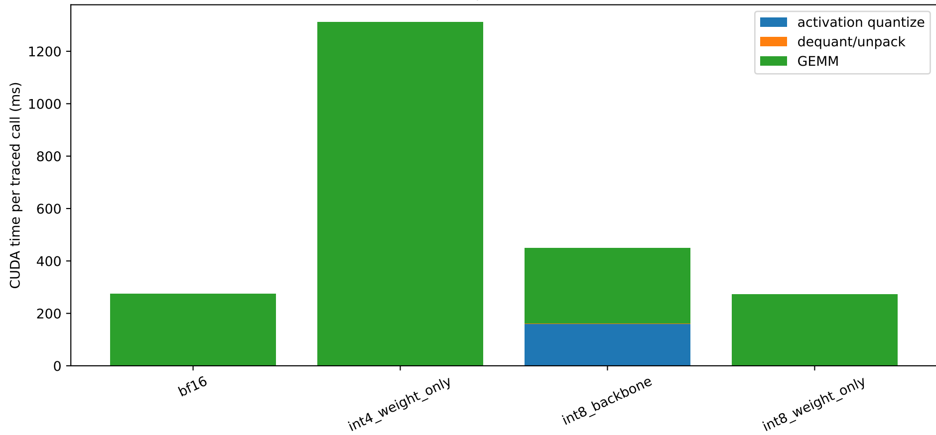
Quantize/dequantize/GEMM time
