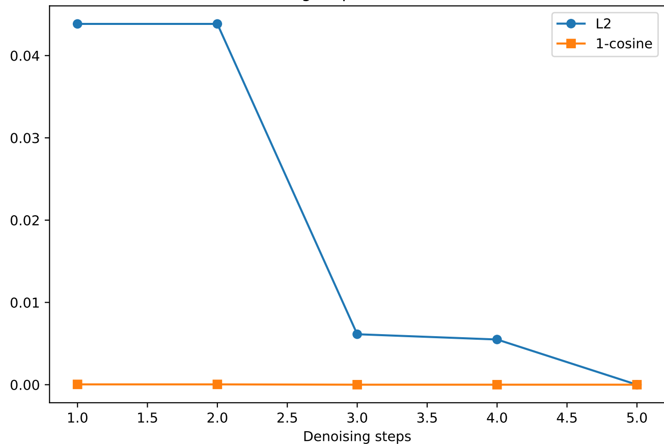
Denoising steps vs action error
