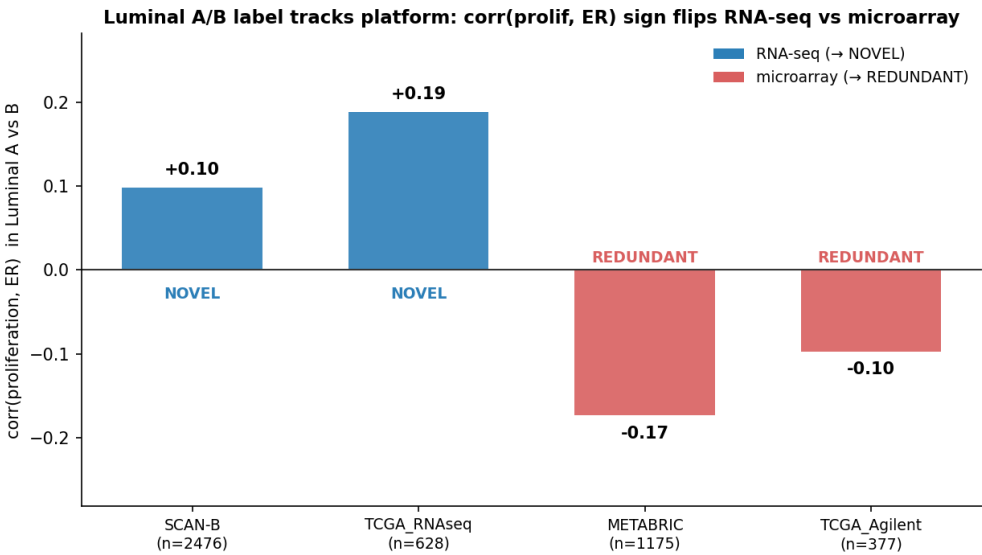
Figure 2: Figure 4. The Luminal A/B platform effect is a sign flip in \text{corr}(\text{proliferation}, \text{ER}) . For the Luminal A vs B endpoint, the proliferation–ER correlation that governs the verdict is plotted per cohort and coloured by platform family. It is positive on the two RNA-seq cohorts (TCGA RNA-seq, SCAN-B) → ER carries unique/suppression variance → NOVEL, and negative on the two microarray cohorts (TCGA Agilent, METABRIC) → ER collinear with proliferation → REDUNDANT. The sign flips even between the two TCGA platforms on the same patients, so it is a measurement property.
