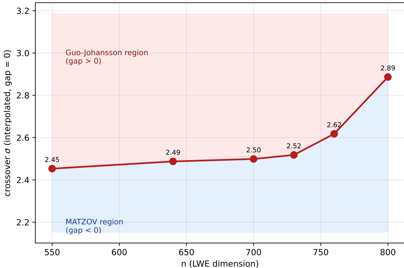
Estimated MATZOV / Guo-Johansson crossover boundary, q = 2^{15}
