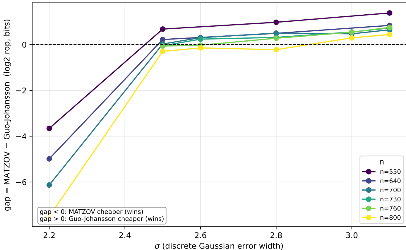
MATZOV vs. Guo-Johansson cost gap across (n, \sigma) , q = 2^{15}
