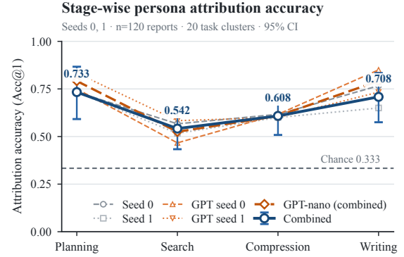
Figure 2: Stage-wise attribution trajectory. Blue (solid): Solar Pro combined ( n = 120 , two seeds) with 95% task-cluster bootstrap intervals; thin grey lines: individual Solar seeds. Orange (dashed): GPT-5.4-nano seed-0 and seed-1 with combined mean. Both evaluators show the same dip-and-recovery shape.
