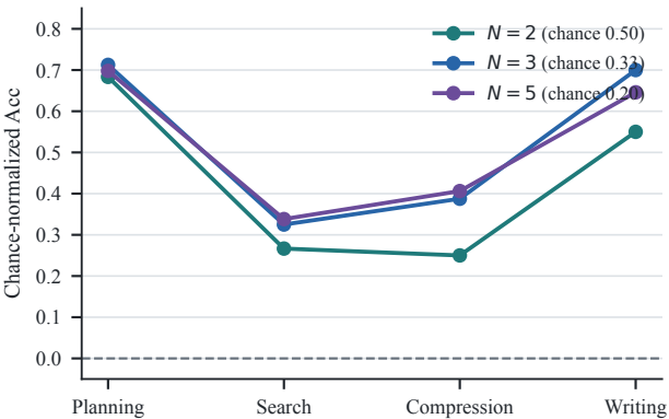
Chance-normalized recoverability by N
