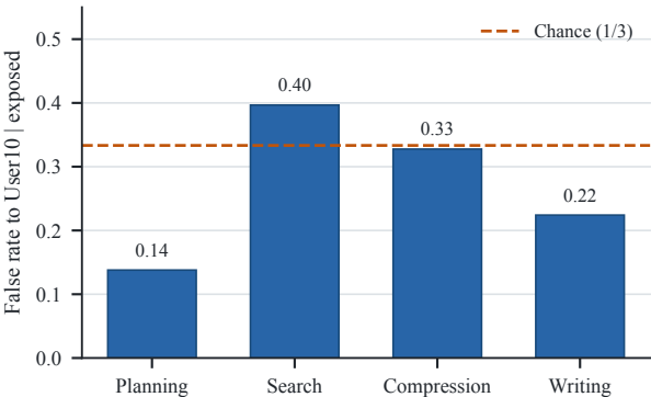
User10 false rate after exposure control
