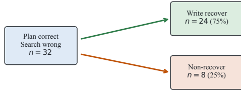
Figure 3: Report-level recovery story for the primary hard-negative protocol: among 32 Plan-correct / Search-wrong reports, 24 (75%) are again correct at Writing and 8 (25%) never recover.
