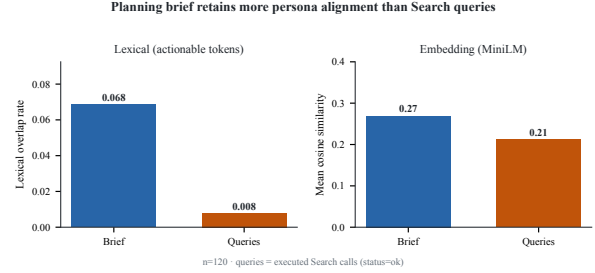
Figure 5: Persona alignment of Planning briefs vs. executed Search queries ( n=120 ). Left: lexical overlap of actionable tokens (0.068→0.008). Right: MiniLM cosine similarity (0.269→0.212). Both drop at query execution; residual embedding alignment separates Search-correct vs. wrong runs (0.236 vs. 0.182).
