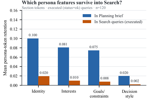
Figure 6: Section-level persona-token retention in Planning briefs vs. executed Search queries ( n=120 ). Identity, interests, and goals/constraints all drop; decision-style language is already sparse in briefs. Field-to-bucket mapping in Appendix L.
