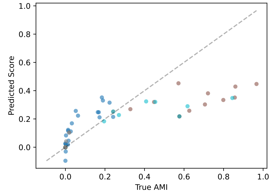
synth_subspace_5of200 Regret=0.395
