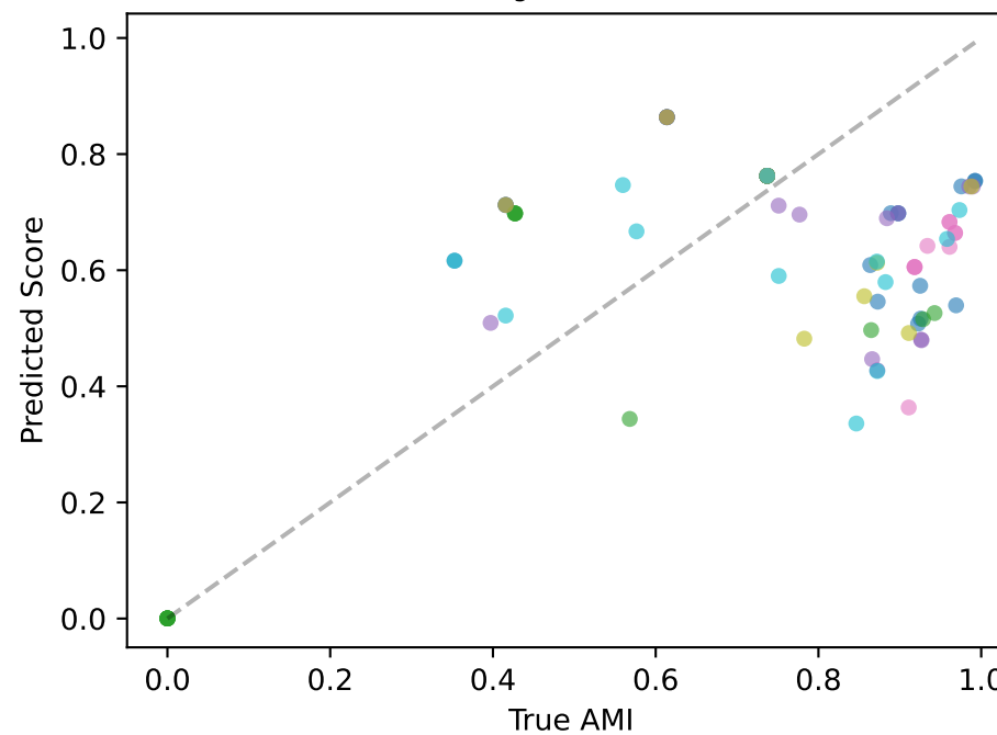
synth_blobs_many_2d Regret=0.379
