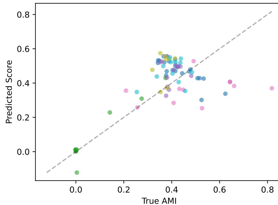
synth_moons_noise0.15 Regret=0.465
