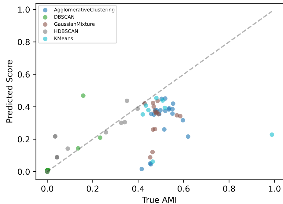
synth_uniform_noise_2d Regret=0.830
