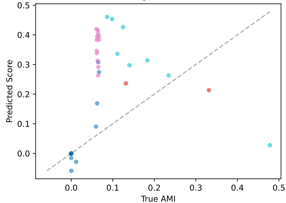
openml_1040 Regret=0.392
