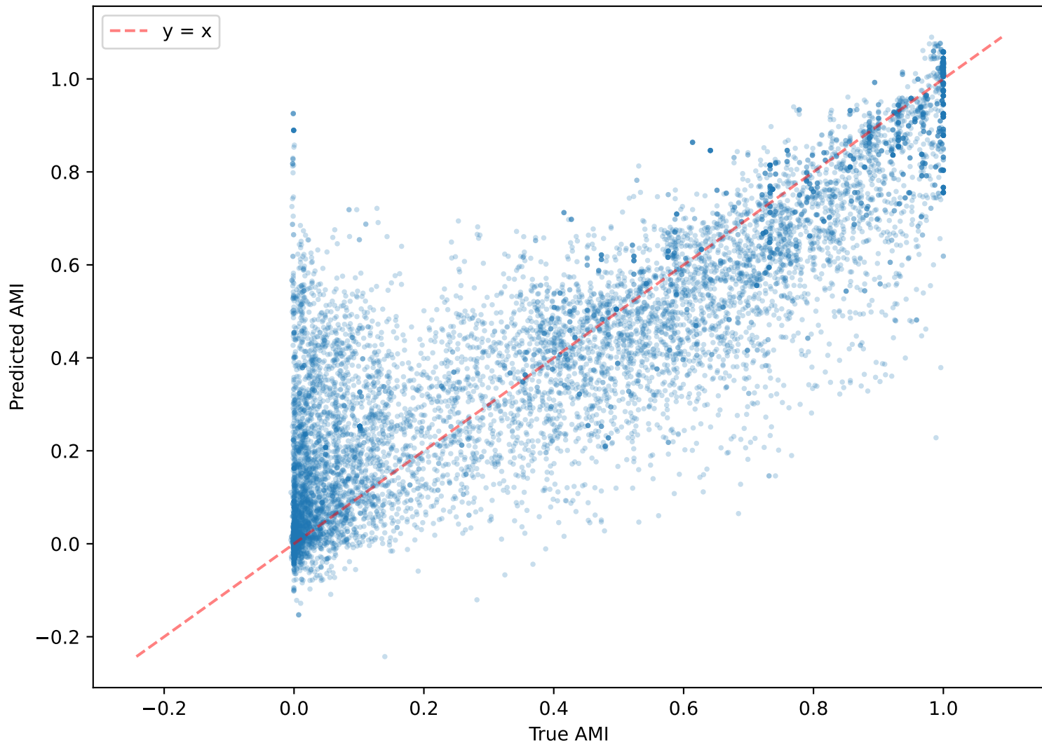
Predicted vs True AMI (all test datasets)
