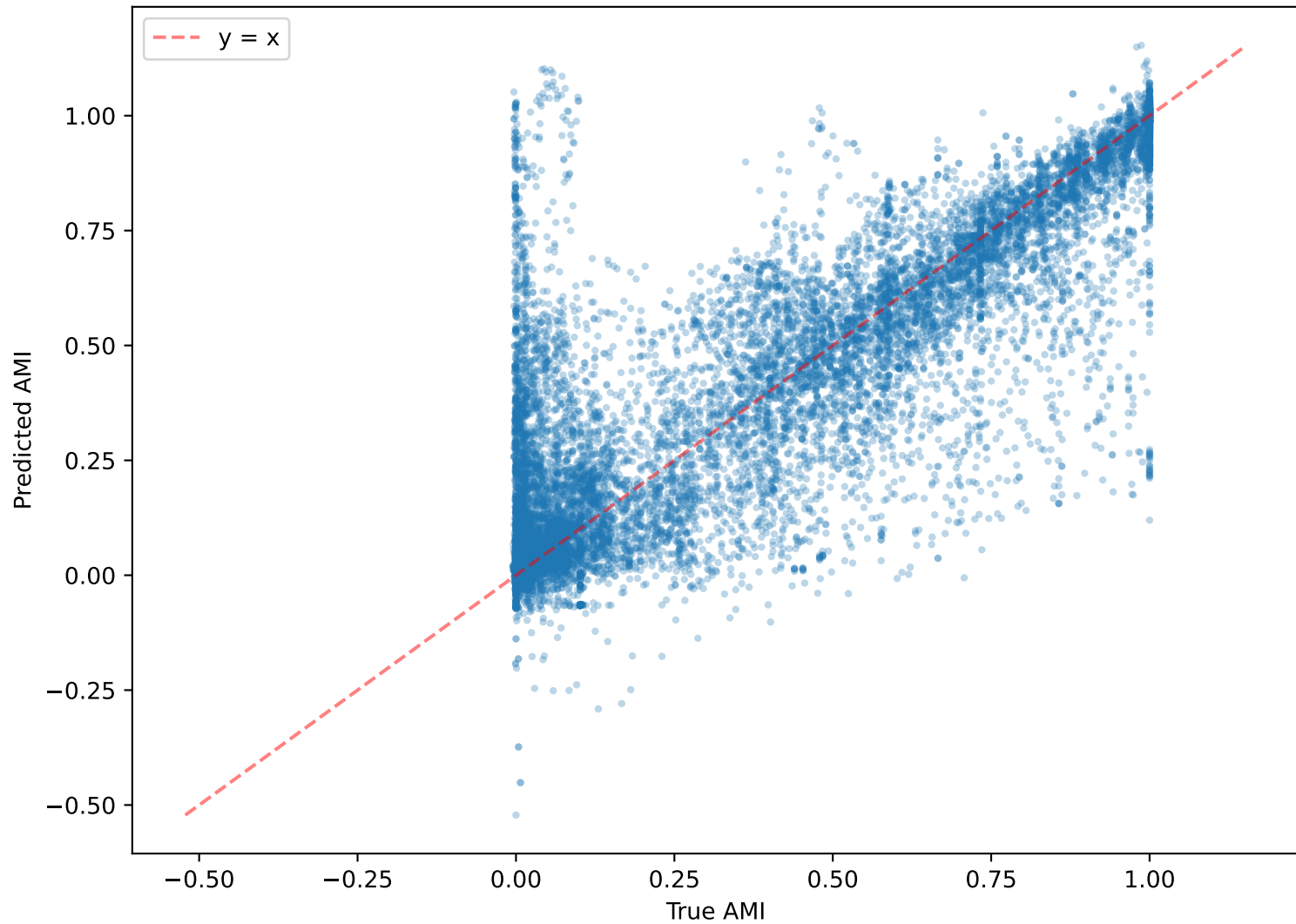
Predicted vs True AMI — MLP (all features)
