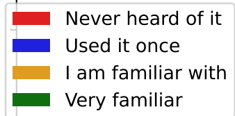
Apptainer Pull
