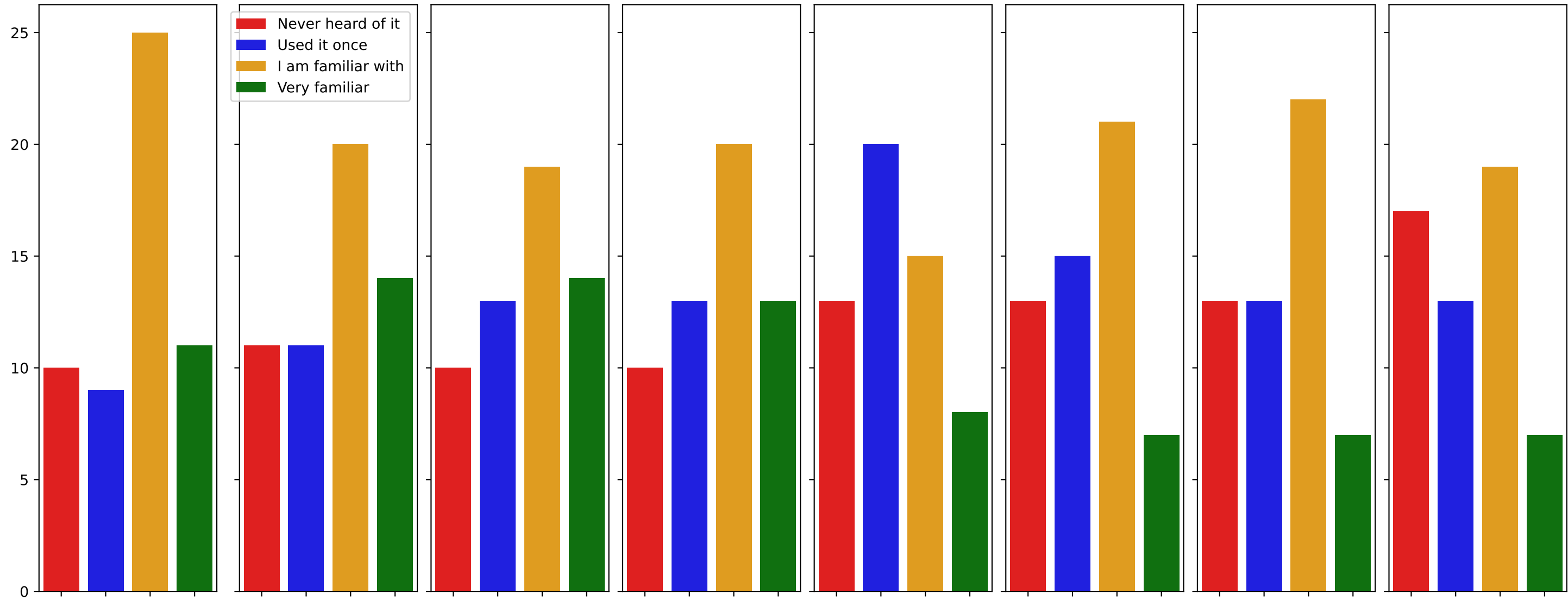
Apptainer Differences
