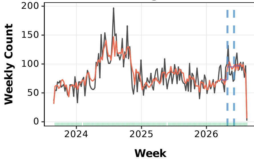
Training Data
