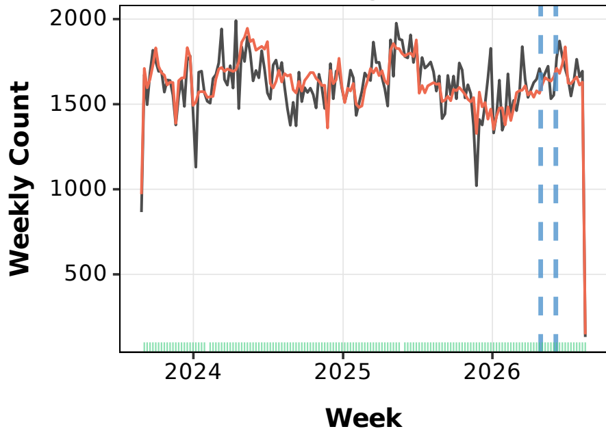
Training Data
