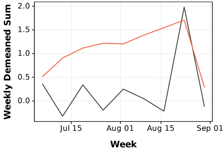
Test Data
