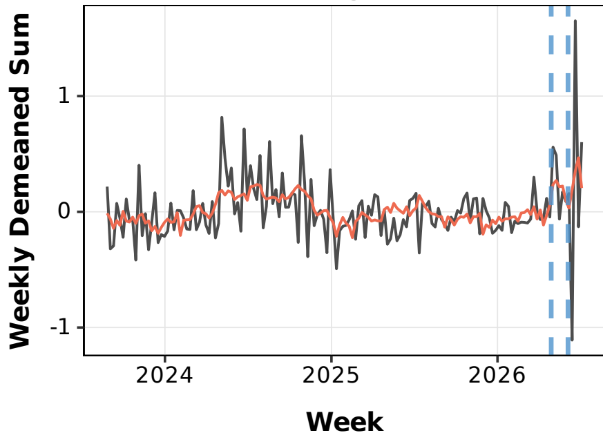
Training Data
