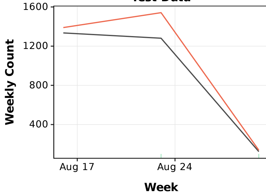
Test Data
