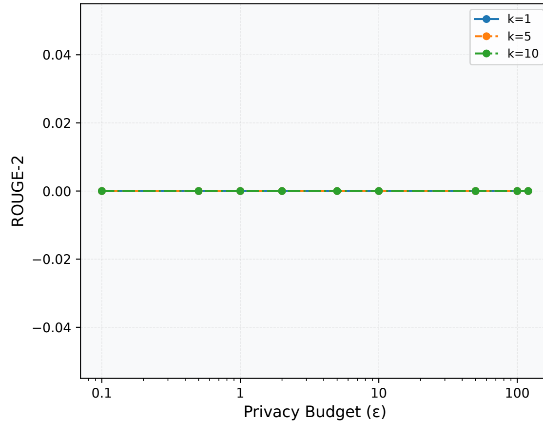
Seed 1
