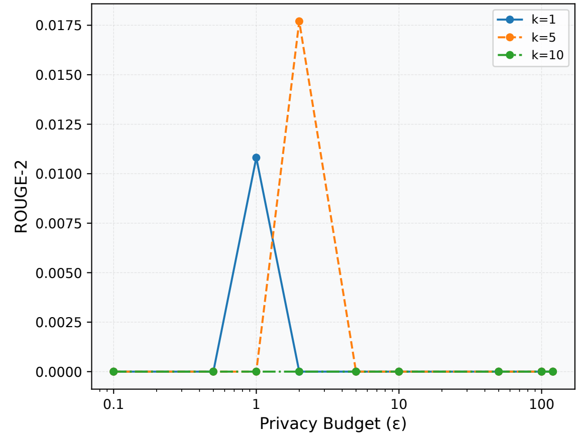
Seed 2
