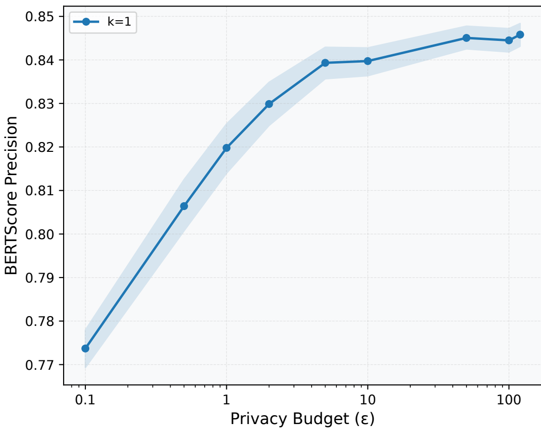
BERTScore Precision
