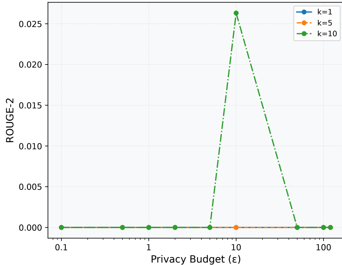
Seed 0
