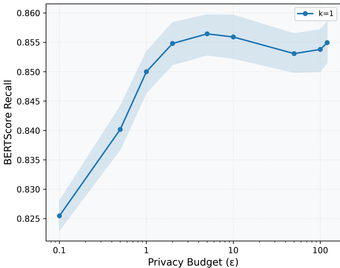
BERTScore Recall
