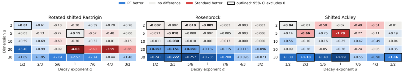
Figure 4: Paired improvement for every dimension and exponent on the three scalable benchmarks.
