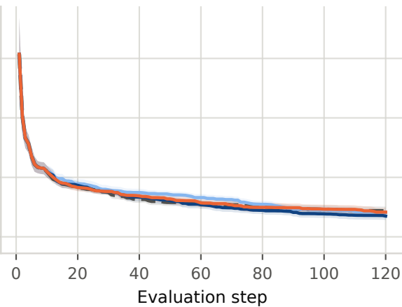
GP-UCB
