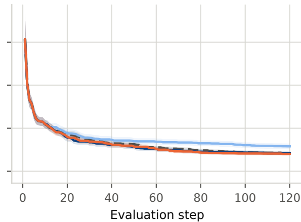
GP-TS
