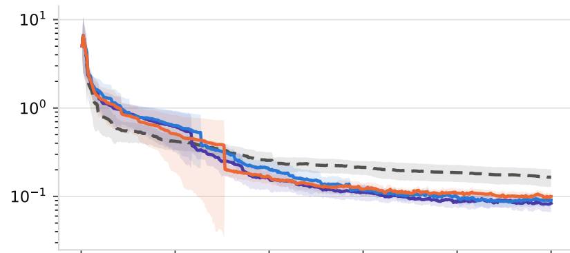
Rosenbrock 30D
