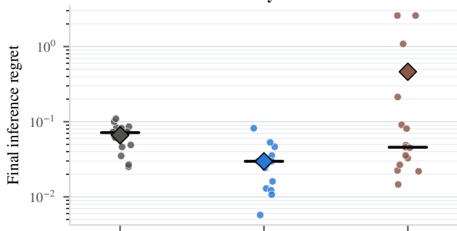
Ackley 2D
