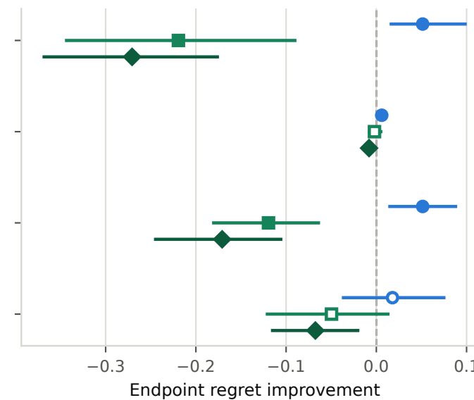
Rosenbrock
