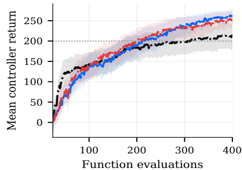
(c) Lunar Lander (12D)
