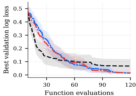
(a) HPO: car (14D)
