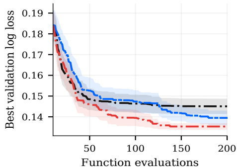
(b) HPO: sylvine (28D)
