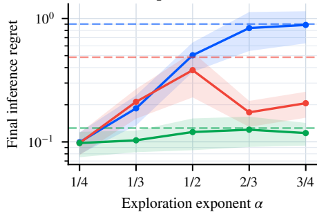
Sphere (30D)
