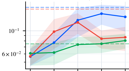
Rosenbrock (20D)
