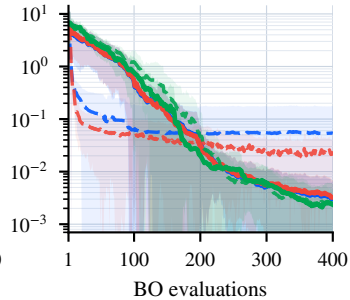
Sum of Different Powers (30D)
