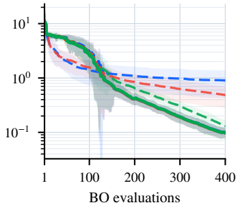
Sphere (30D)
