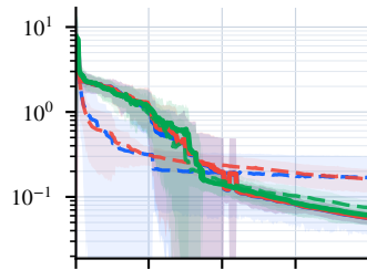
Rosenbrock (20D)
