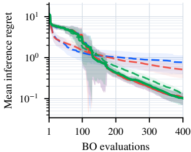
Shifted Bent Cigar (30D)
